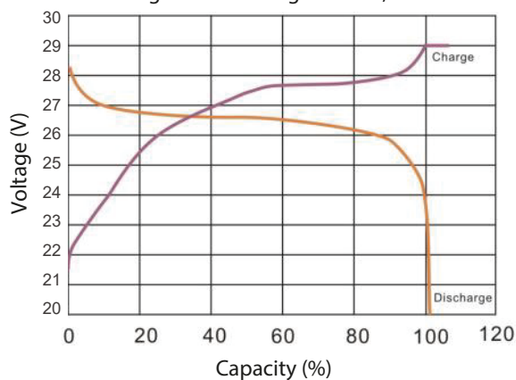
Charge and Discharge at 25°C, 0.2C
